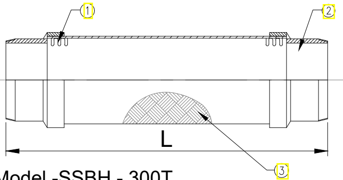
Model -SSBH - 300T THREADED ENDS BSPP / NPT
