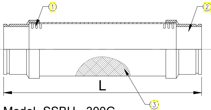
Model -SSBH - 300G GROOVED ENDS
