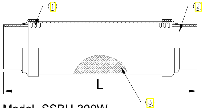
Model -SSBH-300W STEEL WELD ENDS
