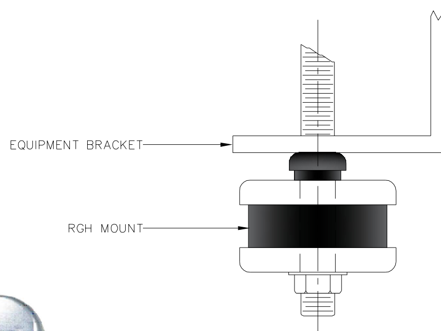
INSTALLED POSITION
