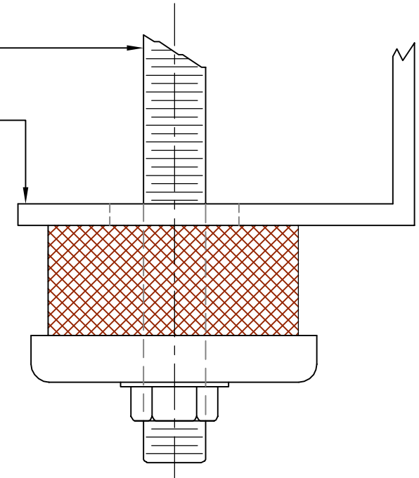
INSTALLED POSITION
