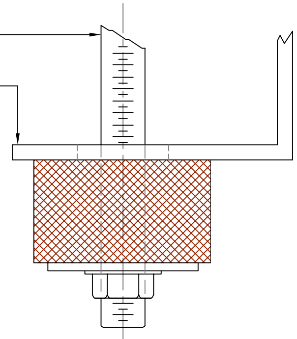
INSTALLED POSITION
